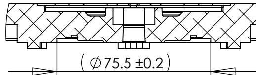
DETAIL B
